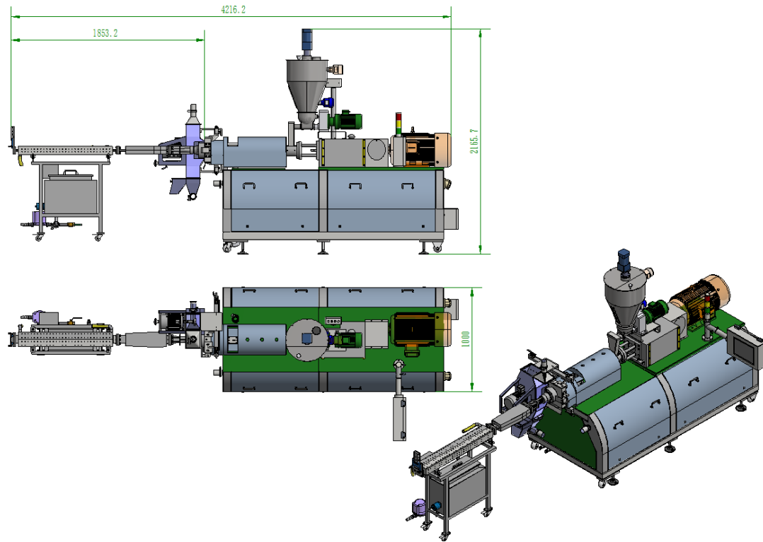
Appendix D. The high-moisture extrusion process designed for developing plant protein-based meat substitutes.
