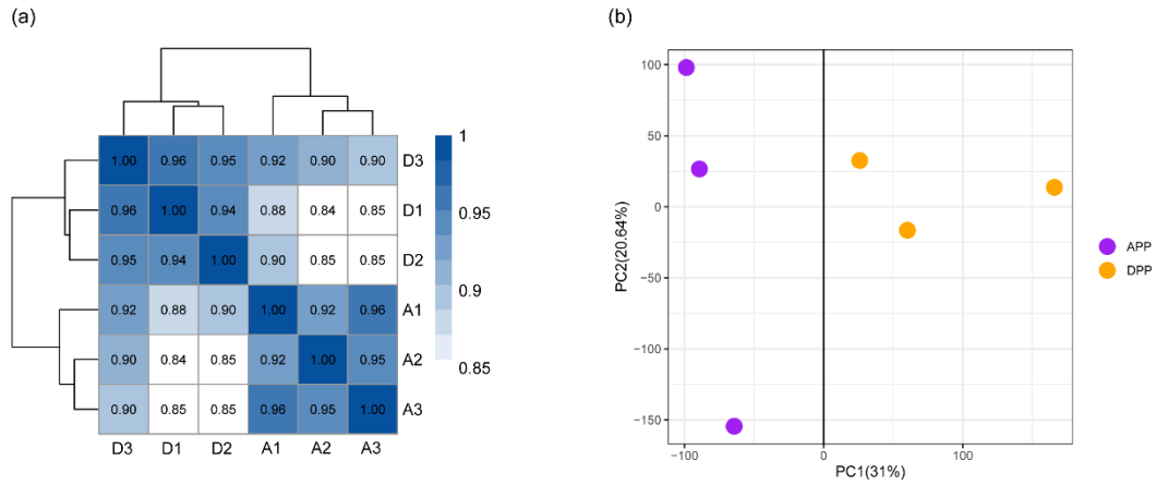
Appendix B. Similarity analysis of RNA-seq samples. (a) Pearson's correlation test and hierarchical clustering for samples. A1-A3: three biological repeats from arborescent phenotype pears (APPs); D1-D3: three biological repeats from dwarf phenotype pear (DPPs). The number in the box represents Pearson's coefficient. (b) Principal component analysis (PCA) of samples based on the gene expression data.
