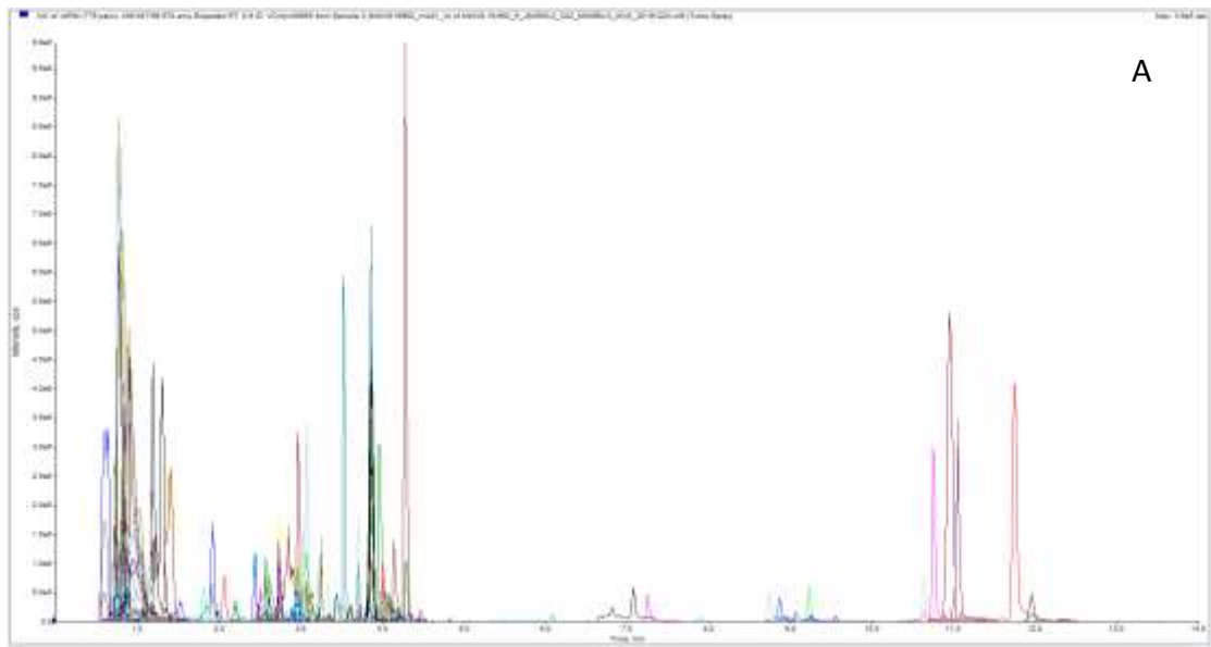
Appendix C. Extracted ion chromatogram (XIC) of mixed quality control samples. A: negative ion mode; B: positive ion mode
