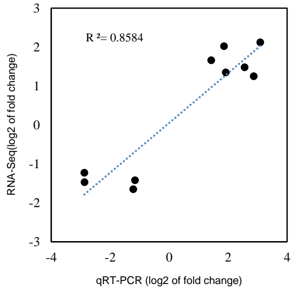
Appendix D Correlation between qRT-PCR and RNA-Seq for the randomly selected genes.
