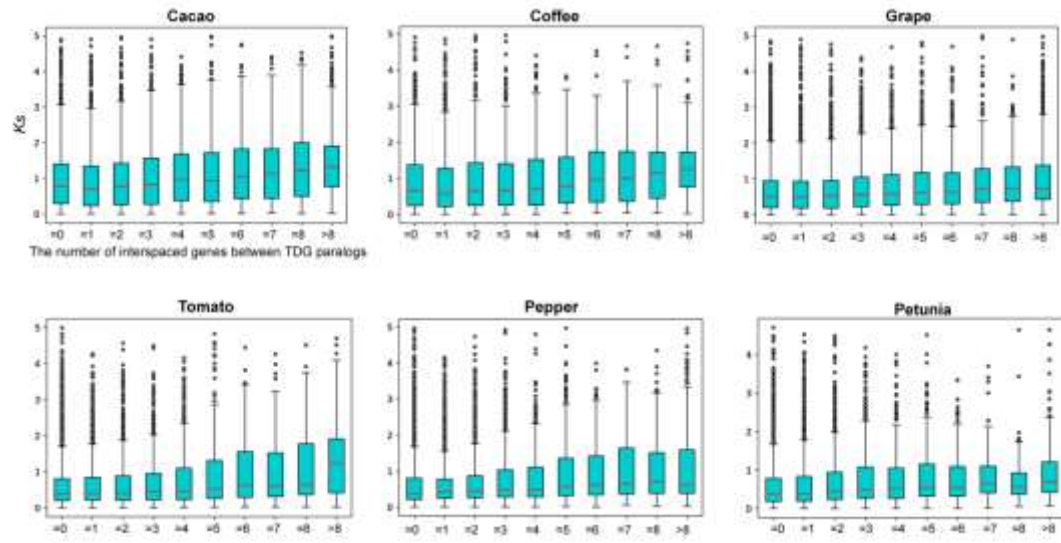
Appendix E The K_s -value of different number of interspaced genes between TDG pairs.
