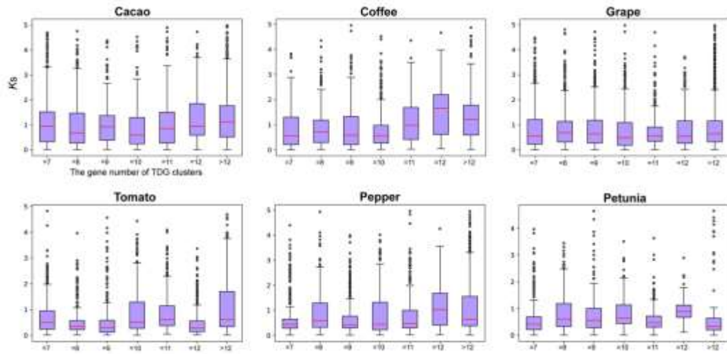
Appendix D In large TDG clusters (gene number > 6), the distribution of K_S -values in TDG clusters with different numbers of genes.
