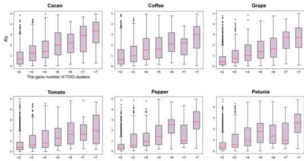
Appendix C The distribution of the largest K_s -values in TDG clusters with different number of genes.
