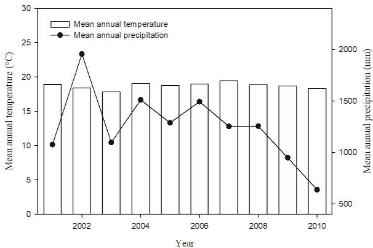
Fig. S1 Mean annual temperature (MAT) and mean annual precipitation (MAP) during cultivation period at experimental site.
