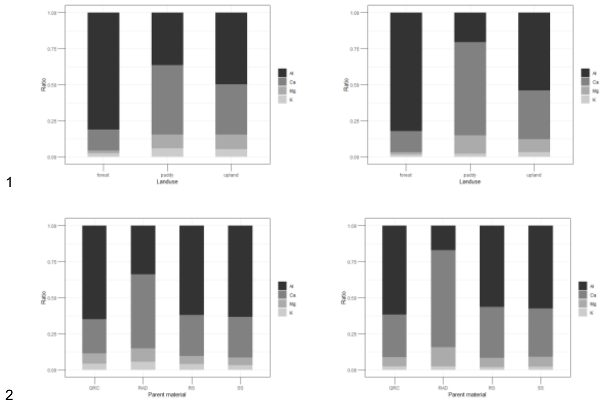
3 Fig. S1 Relative percentages of exchangeable cations (Al, Ca, Mg and K) under 4 different land use types (A, B) and parent materials (C, D) in the surface layer (A, C) 5 and subsurface layer (B, D) in Yujiang.
