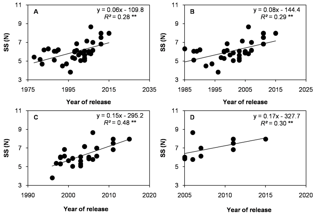
Appendix C Changes of stem strength of 40 wheat cultivars over breeding periods of 1975-2015 (A), 1985-2015 (B), 1995-2015 (C) and 2005-2015 (D), respectively. SS: stem strength.
