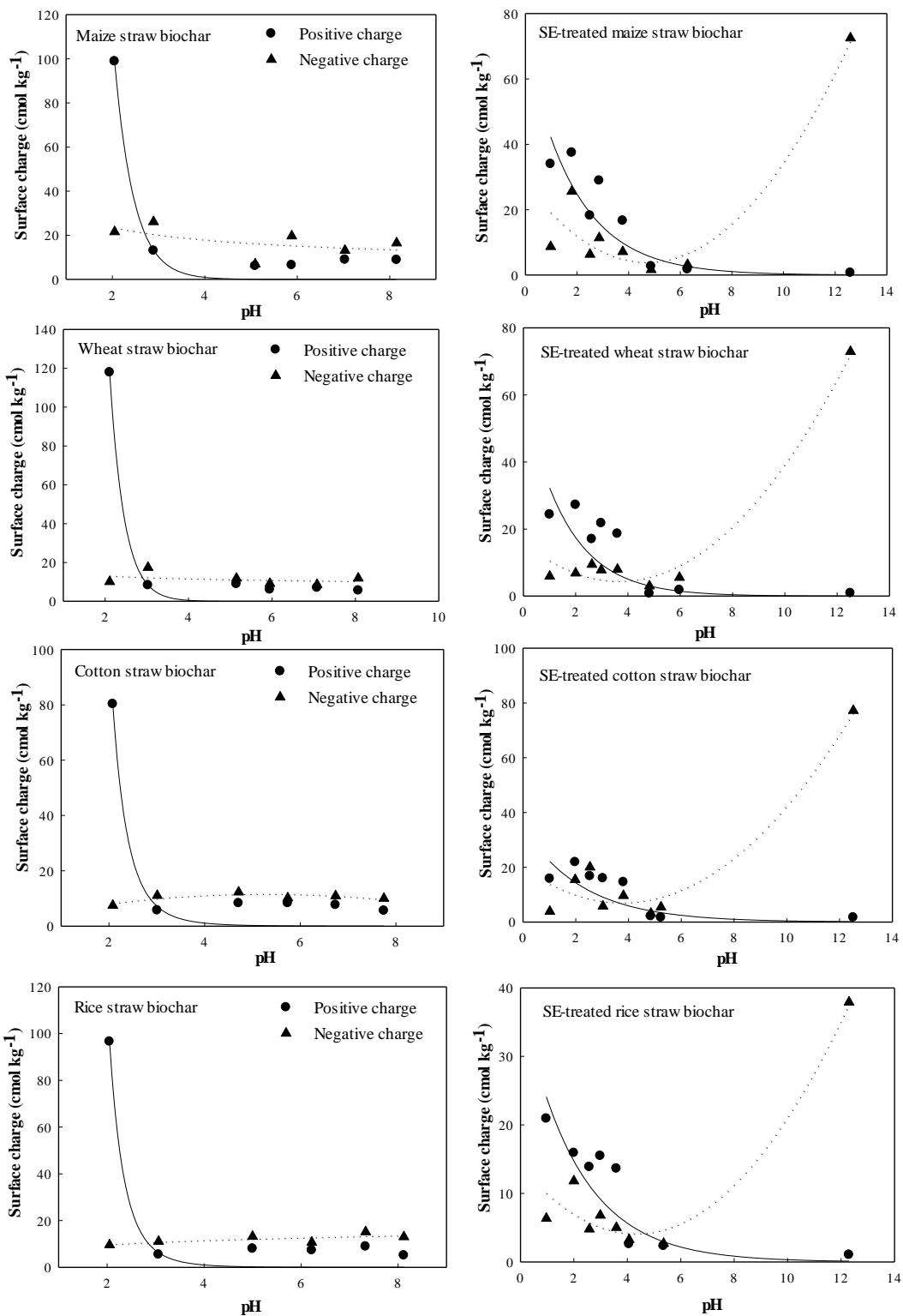
Changes in surface positive and negative charges with medium pH values for the biochars derived from different pristine and steam-exploded (SE) crop straws.
