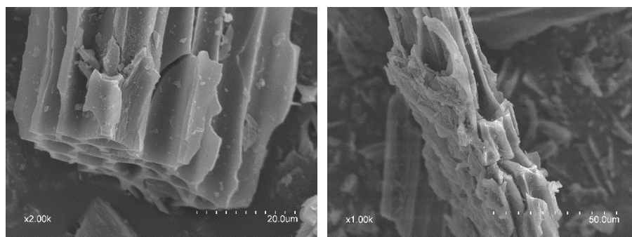
SEM images of the biochars derived from pristine ( left ) and steam-exploded ( right ) crop straws.
