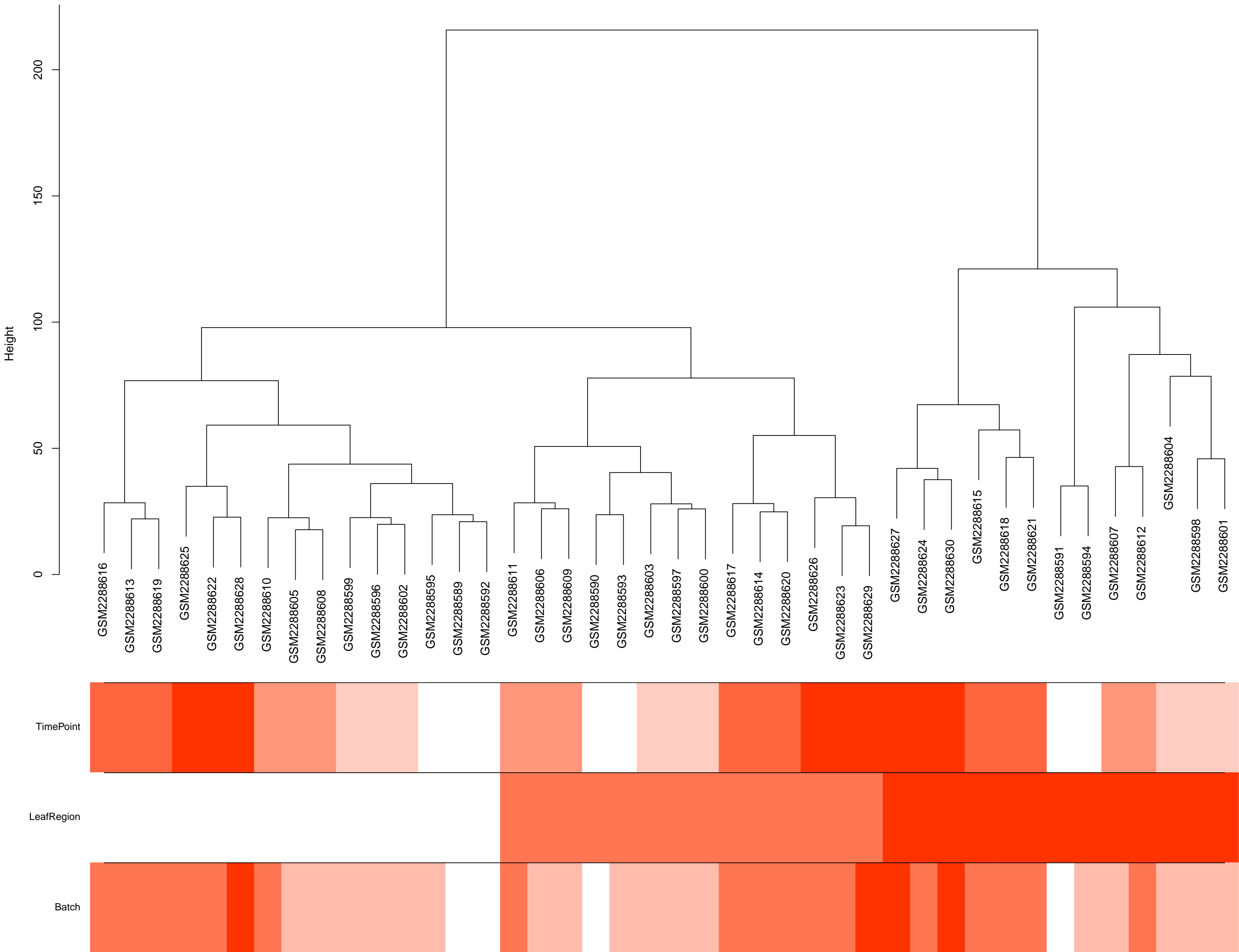
Sample dendrogram and Info heatmap
