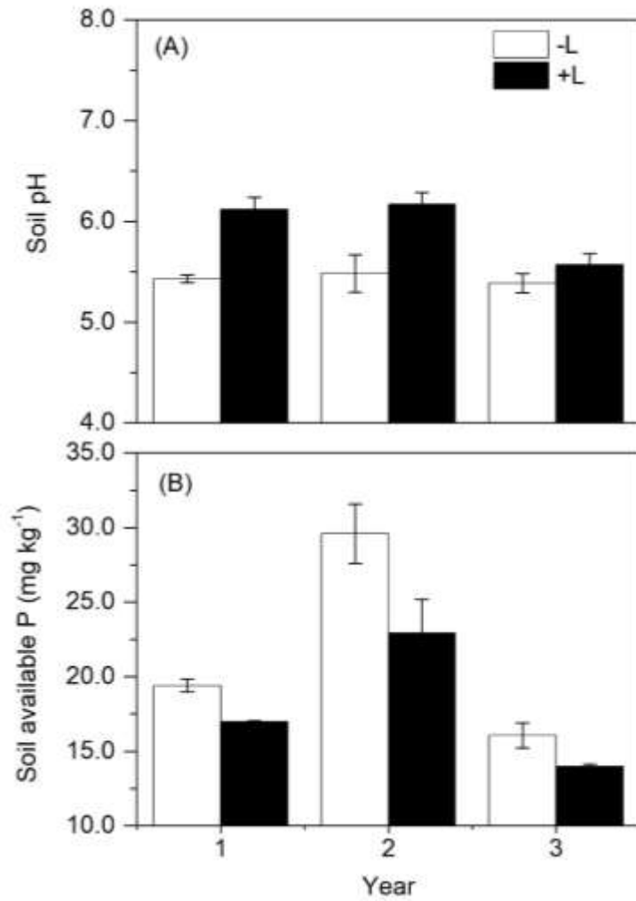
Appendix C Soil pH and soil available P as affected by liming (-L and +L) for years 1-3 in our study (2015-2017). Error bars represent the 95% confidence interval (CI) of the mean.
