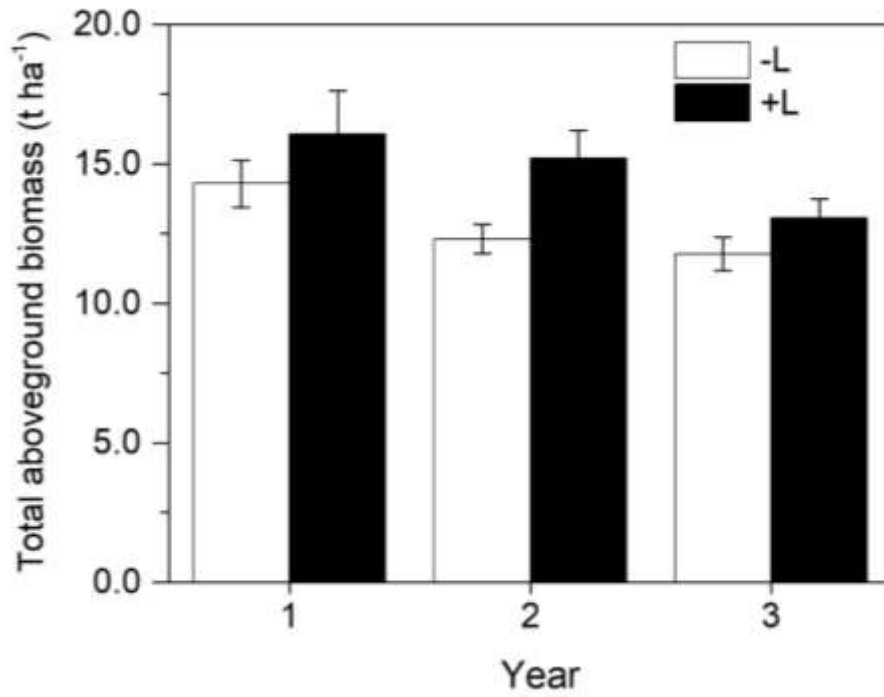
Appendix A Total aboveground biomass as affected by liming (-L and +L) and years (2015-2017). Error bars represent the 95% confidence interval (CI) of the mean.
