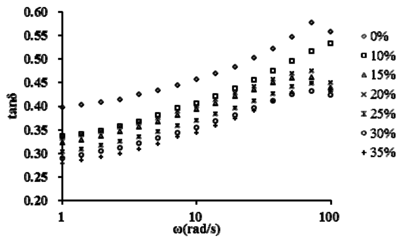
Appendix A Mechanical spectra (a and b) and tangent of phase shift (c) of wheat dough with different potato flour proportions.
