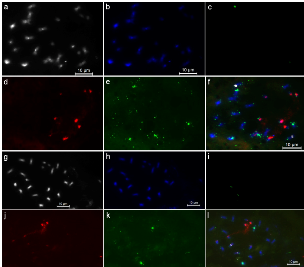
Appendix C Sequential FISH of A. duranensis (a-f) and A. ipaënsis (g-l). a and g , DAPI staining (gray white); b and h , blue, DAPI staining ; c and I , green, 5S rDNA labeled with biotin-16-dUTP and detected with fluorescein anti-biotin; d and j , red, 45S rDNA labeled with digoxigenin-11-dUTP and detected with anti-digoxigenin-rhodamine; e and k , green, (TTTAGGG) n labeled with biotin-16-dUTP and detected with fluorescein anti-biotin; f and I , merged of b to e and g to k, white (the original green signals of 5S rDNA were converted to pseudo color white), 5S rDNA; red, 45S rDNA; green, telomeric repeats (TTTAGGG) n .
