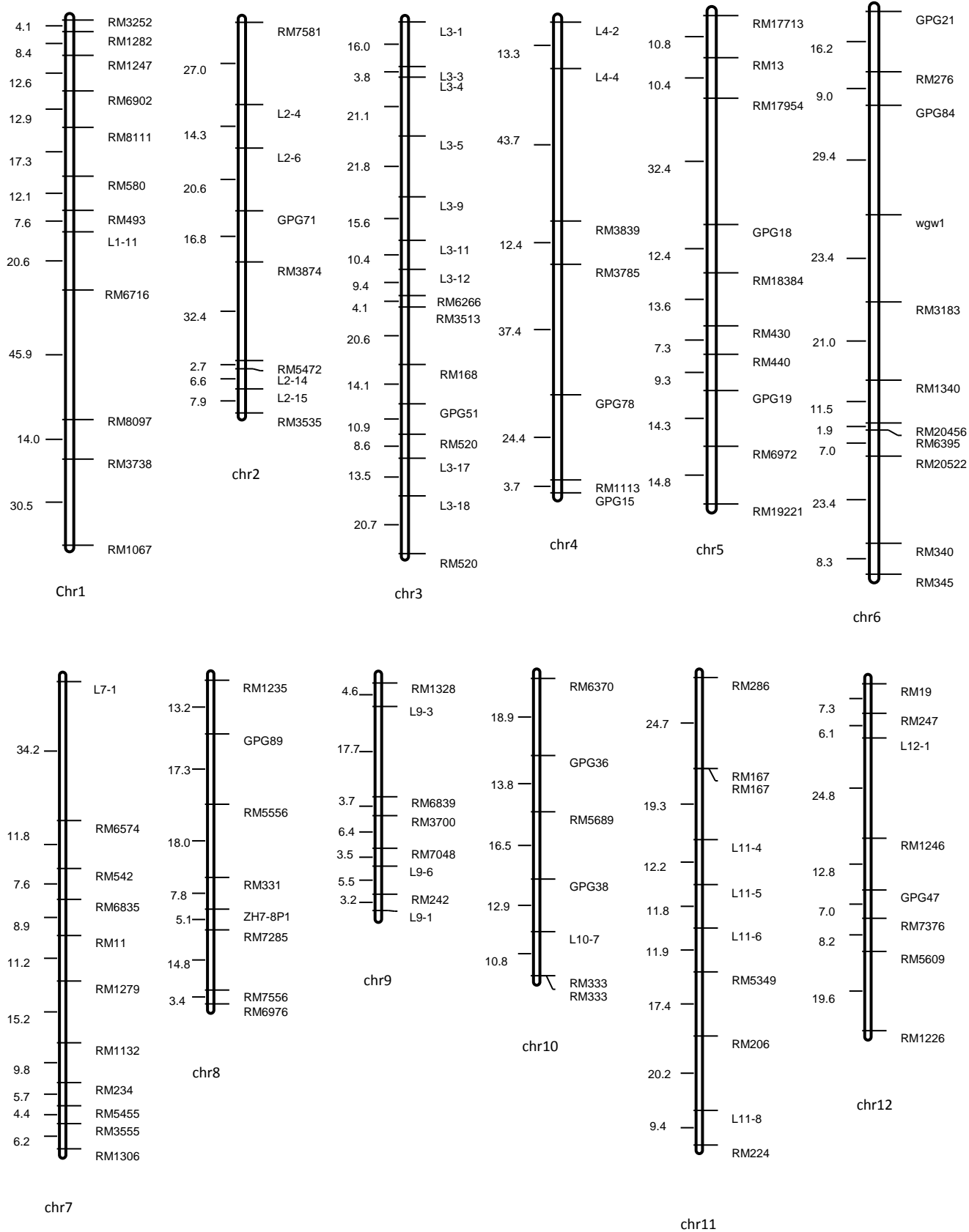
Supplemental Figure 1. A genetic linkage map
