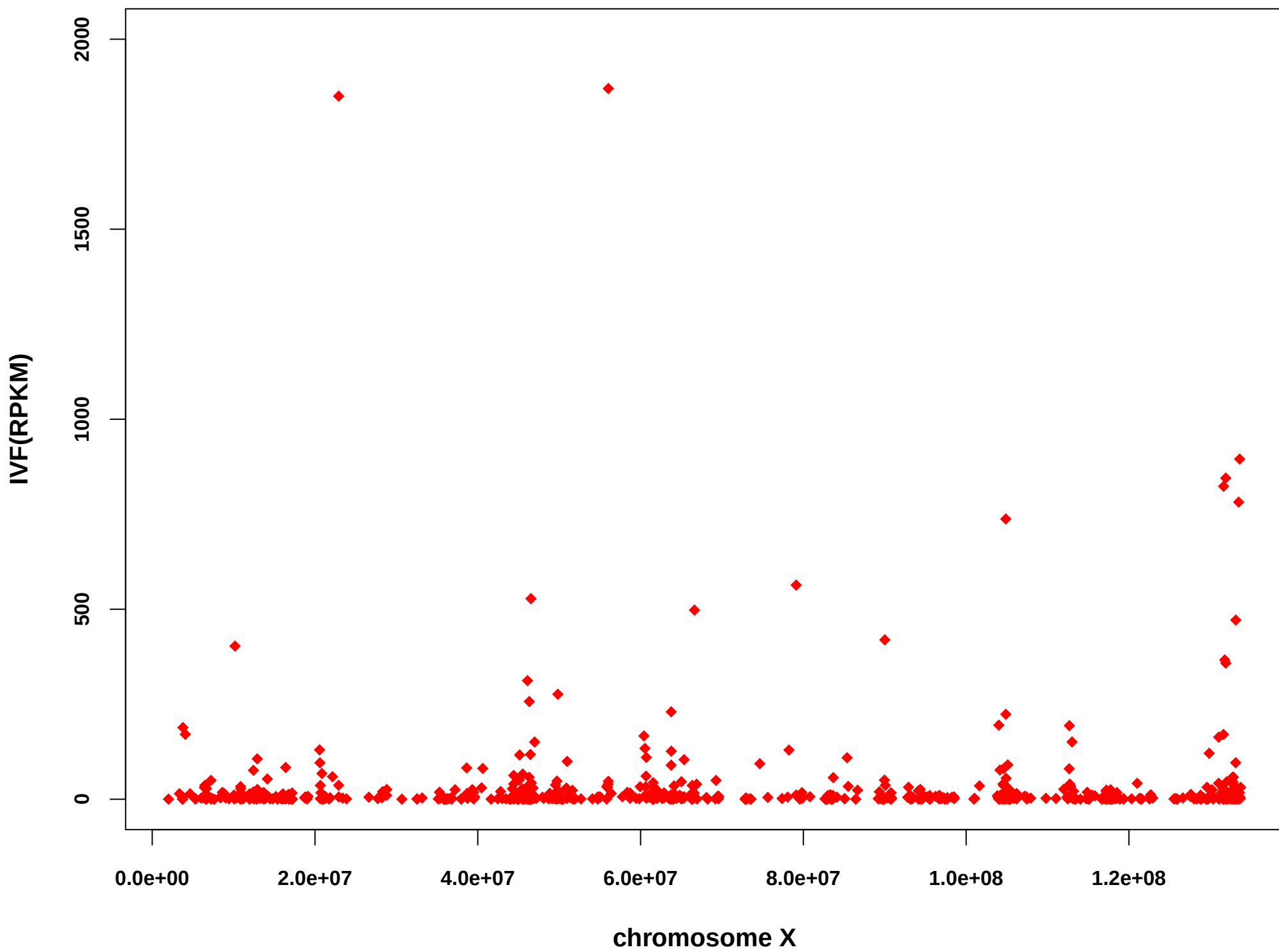
Distribution of IVF(RPKM) on Chromosome X
