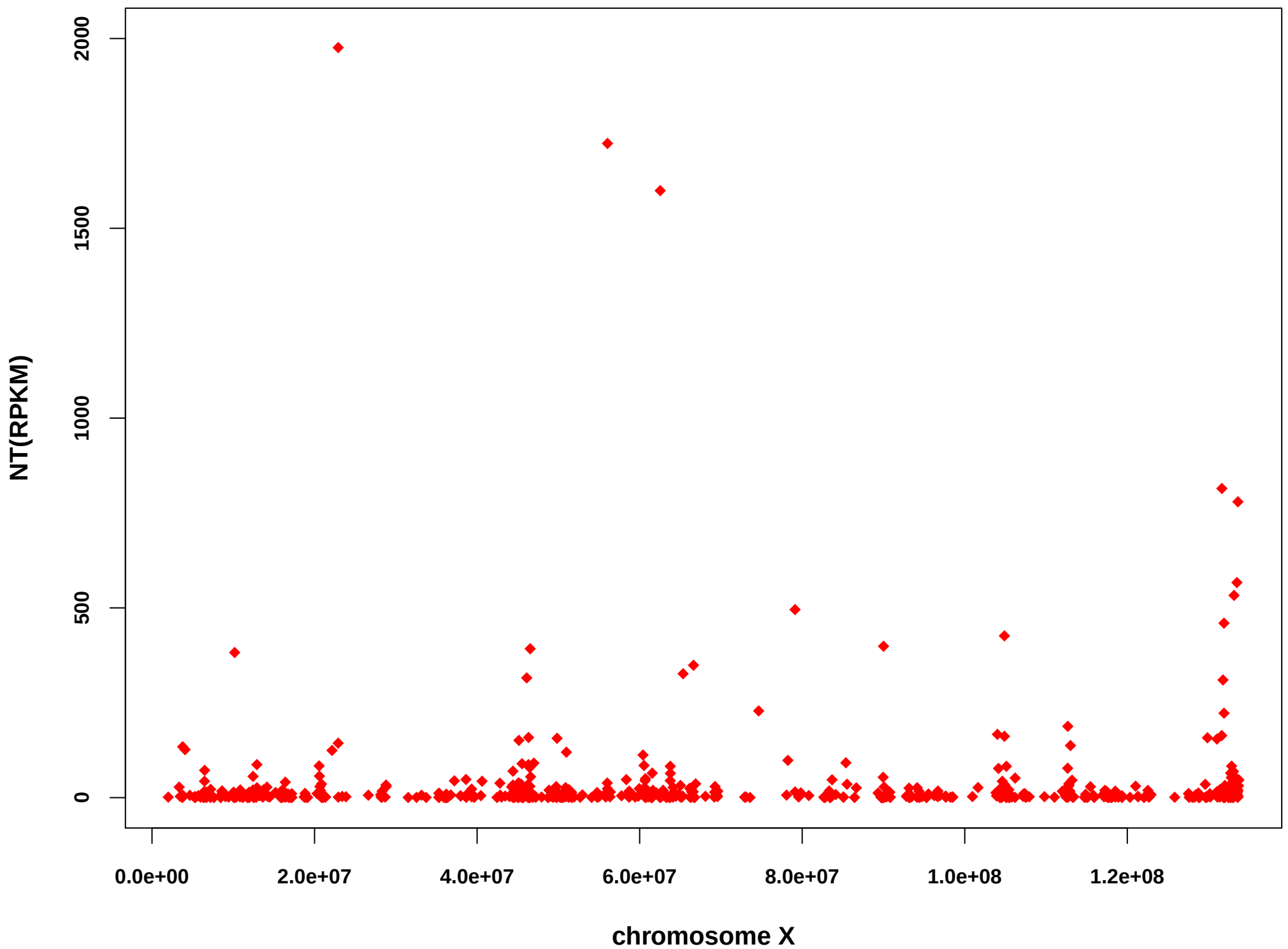
Distribution of NT(RPKM) on Chromosome X
