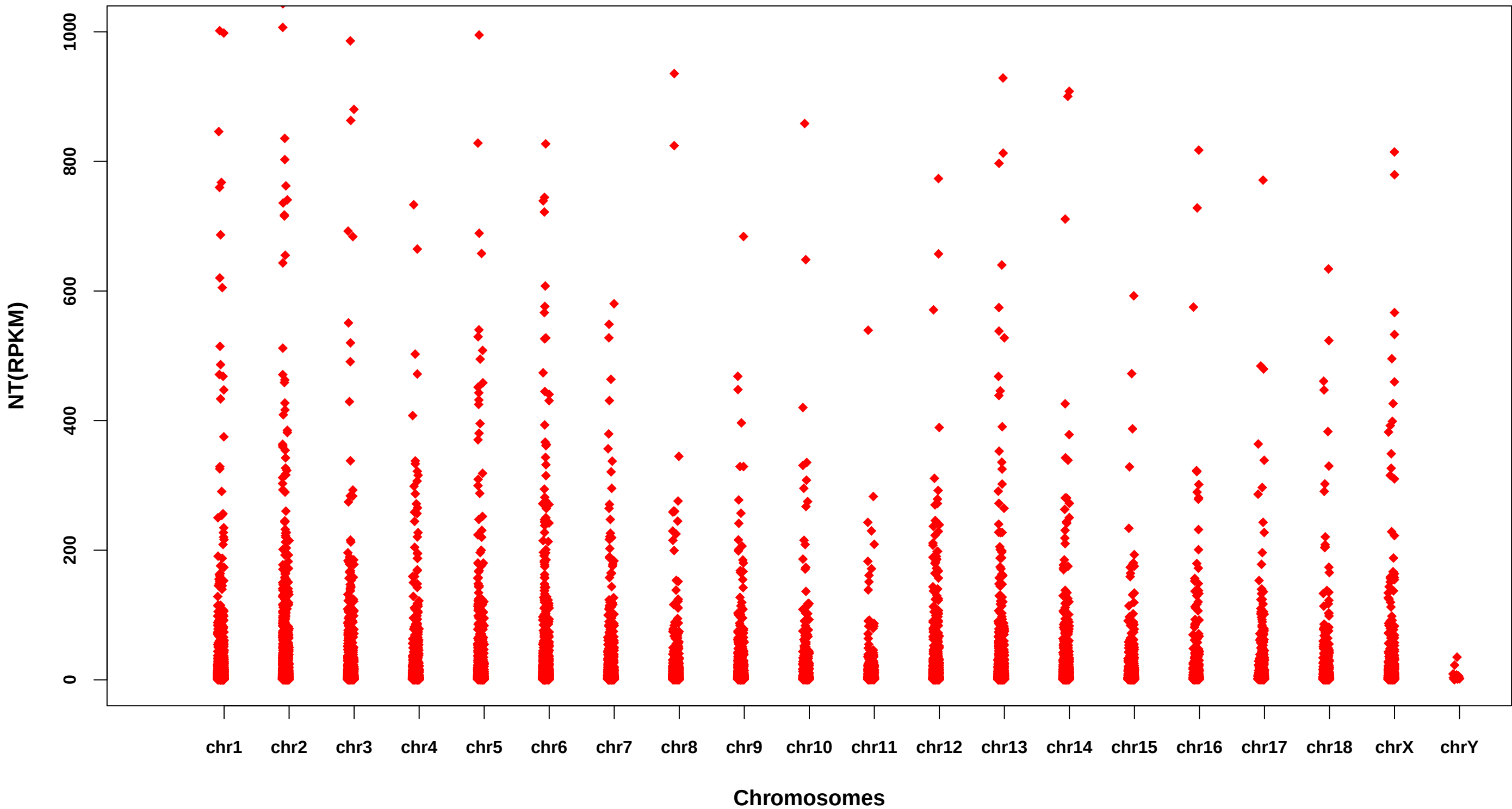
Distribution of NT(RPKM) on Chromosomes
