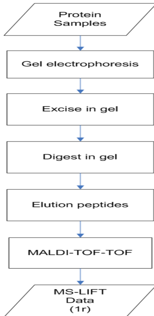
Appendix C Identification process of protein spots in this study.
